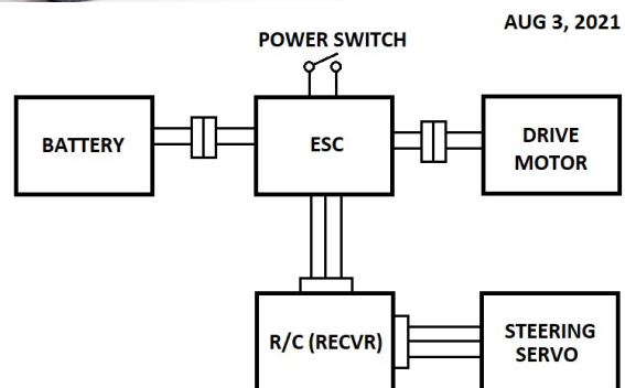
SCHEMATIC - M3 HALFTRACK
